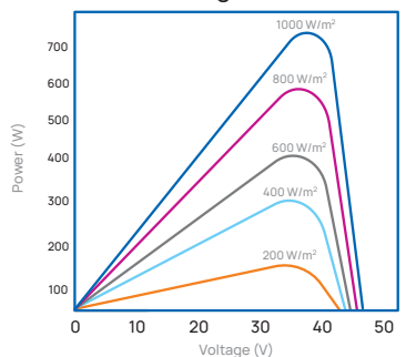
Power-Voltage Curve 725W
